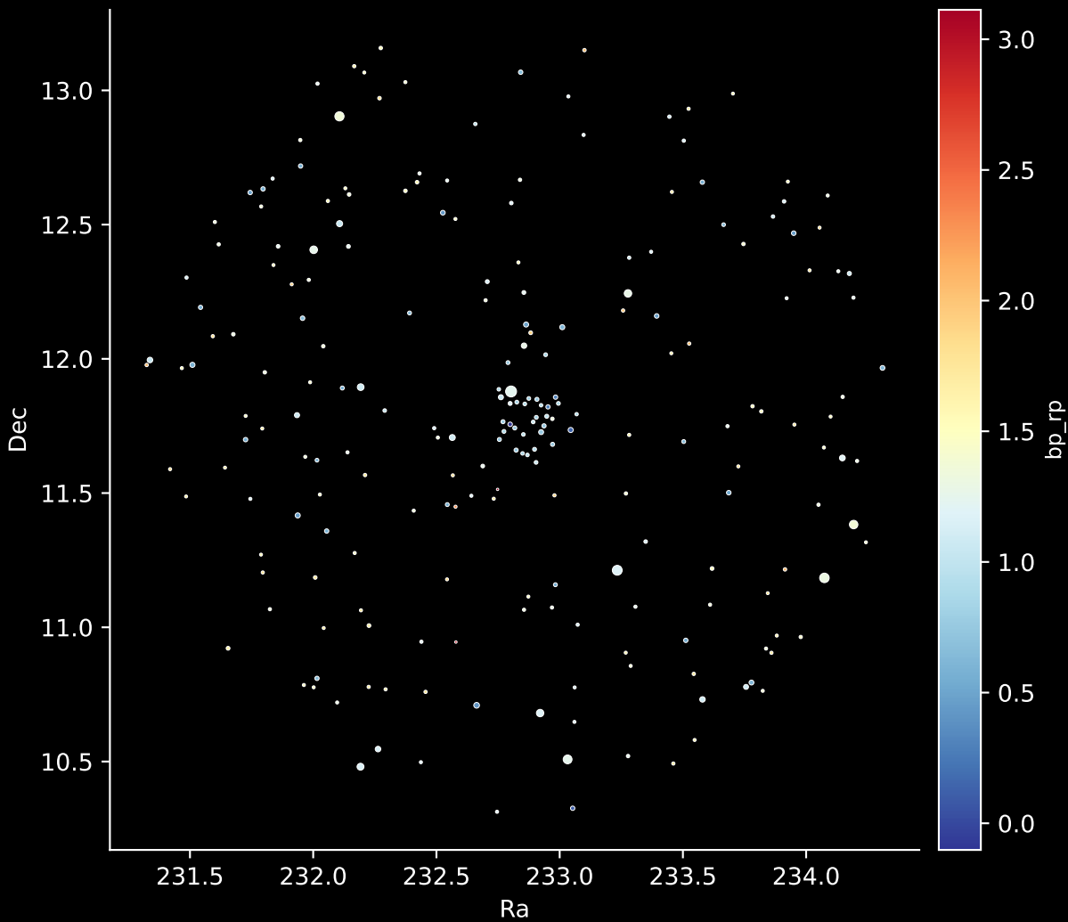
APOGEE DR17 Field: [M67-RV] Stars: 224
